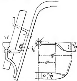
Figs. 2996-2997. Bracket for Lubricator Drip Cup.
